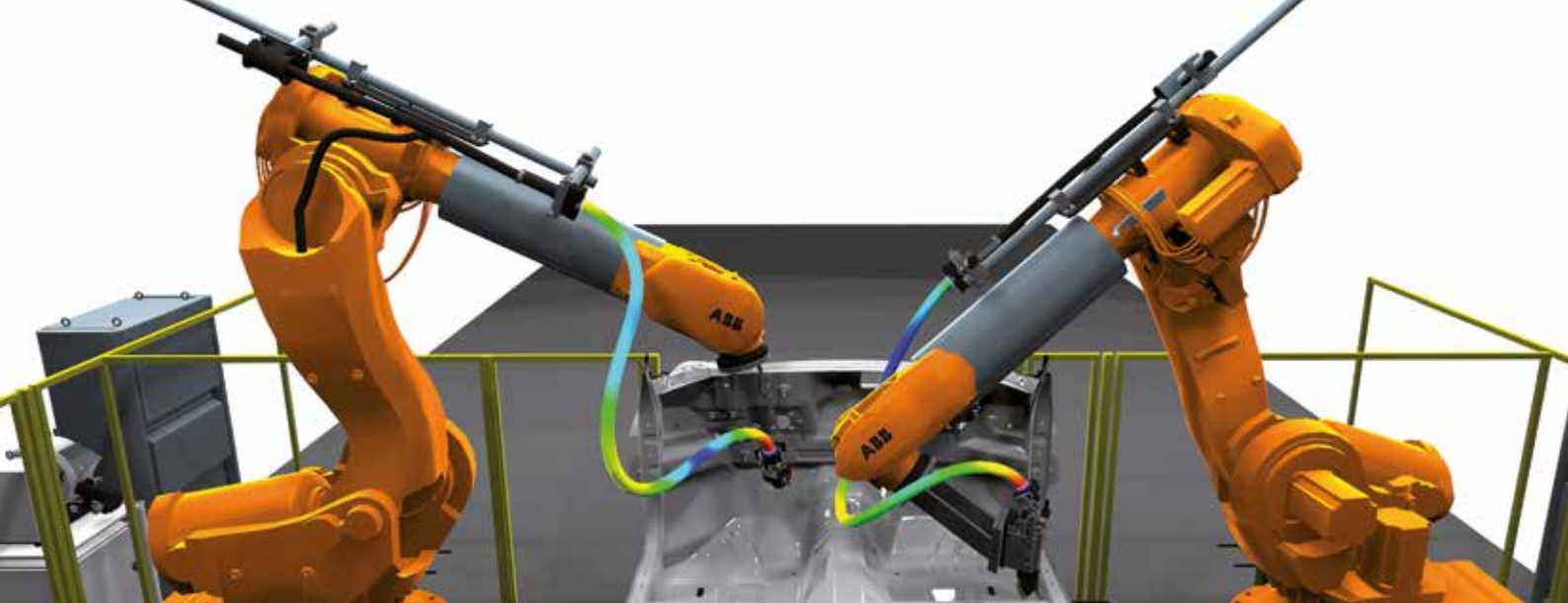
Virtual wiring system design of a Volvo XC 90 with IPS cable simulation
